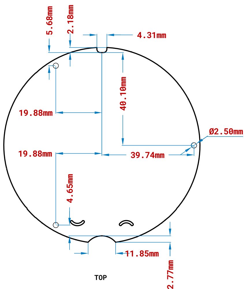
Mechanical view
